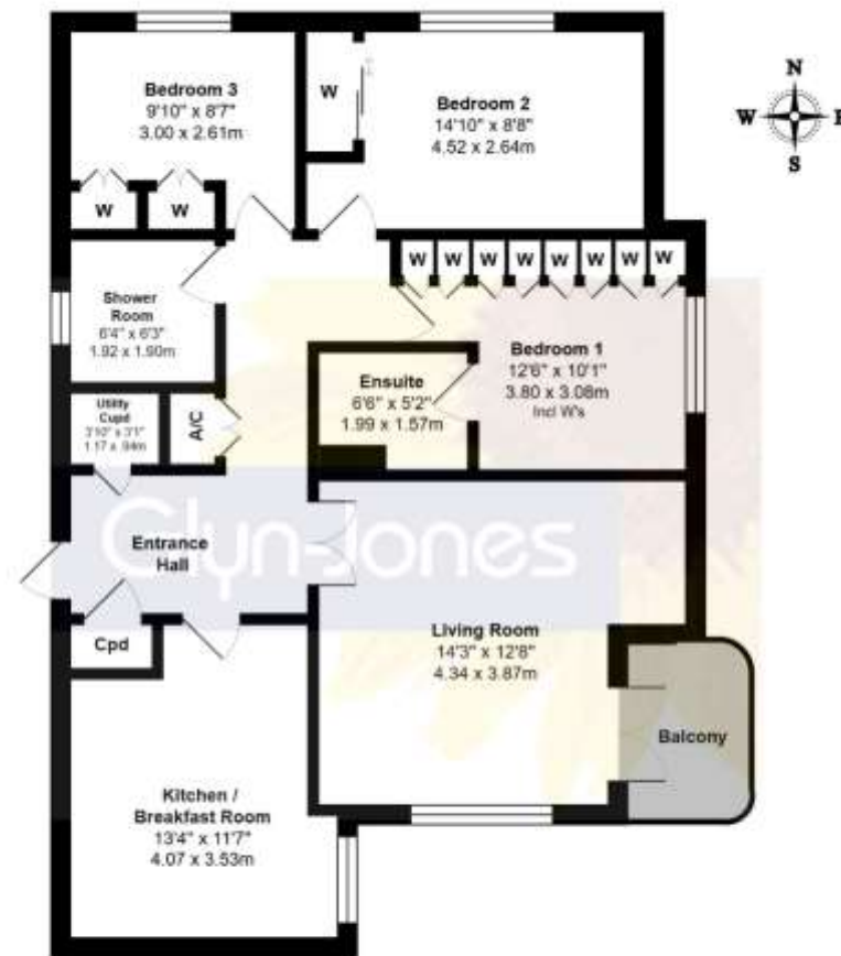
Second Floor
