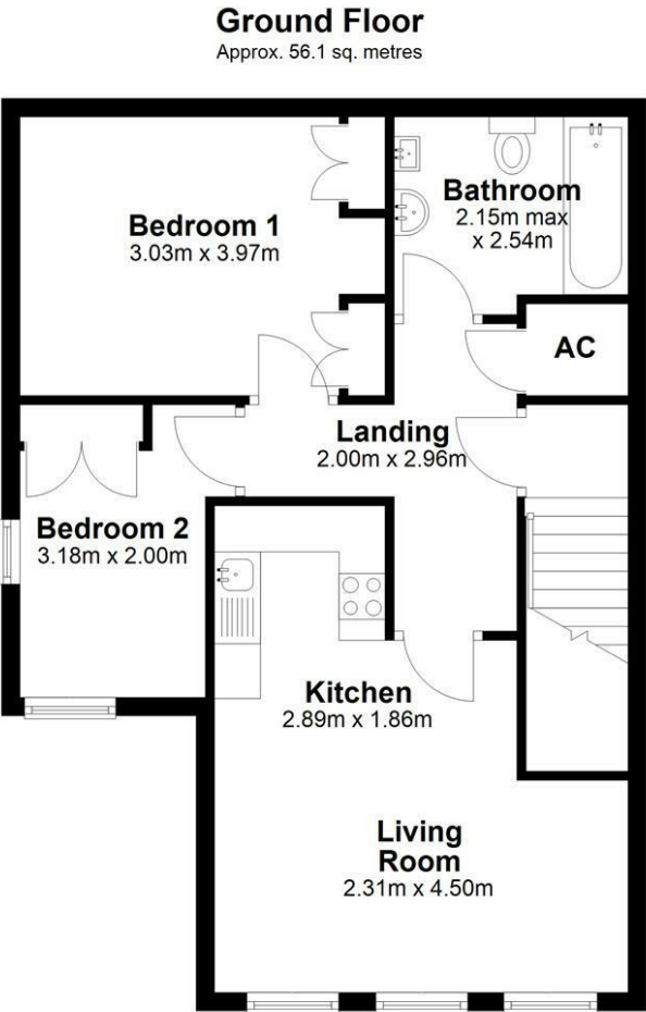
Total area: approx. 56.1 sq. metres Andros, Leigh Road, Chulmleigh, Devon
