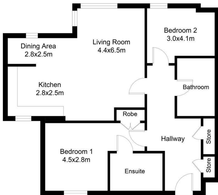
FLOOR PLAN
