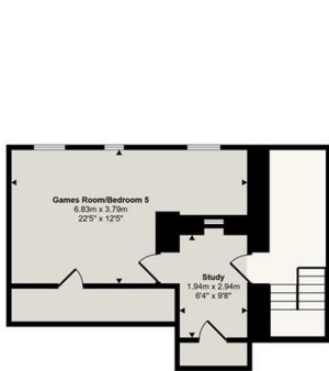
Cellar Approx 48 sq m / 517 sq ft
