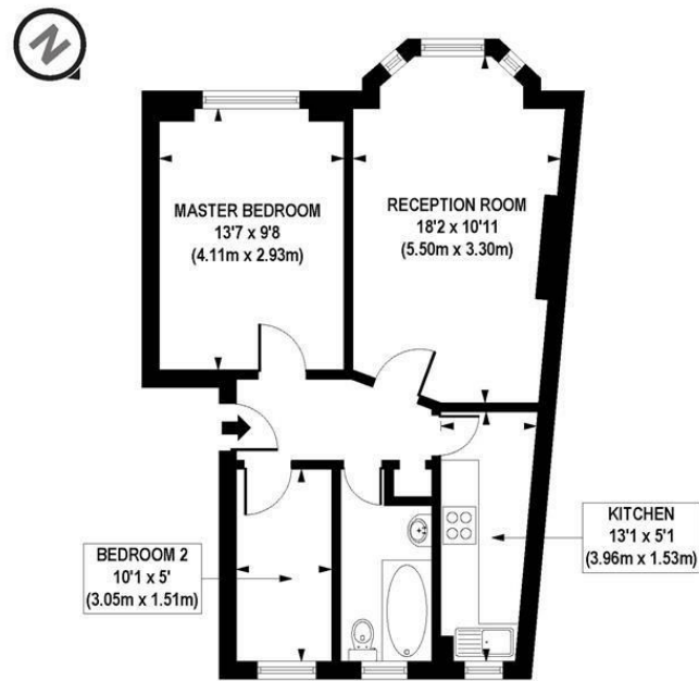
THIRD FLOOR
