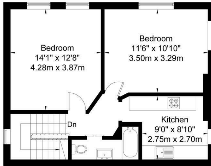
Third Floor
