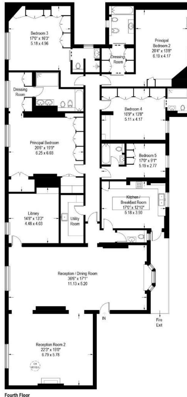
Fourth Floor
