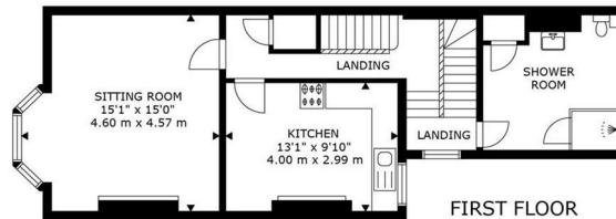
FIRST FLOOR
